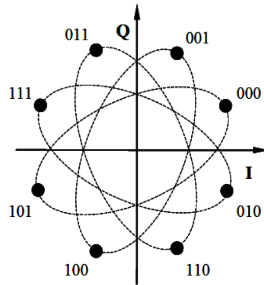
8-EPSK
