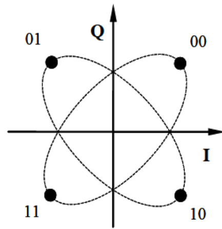
4-EPSK
