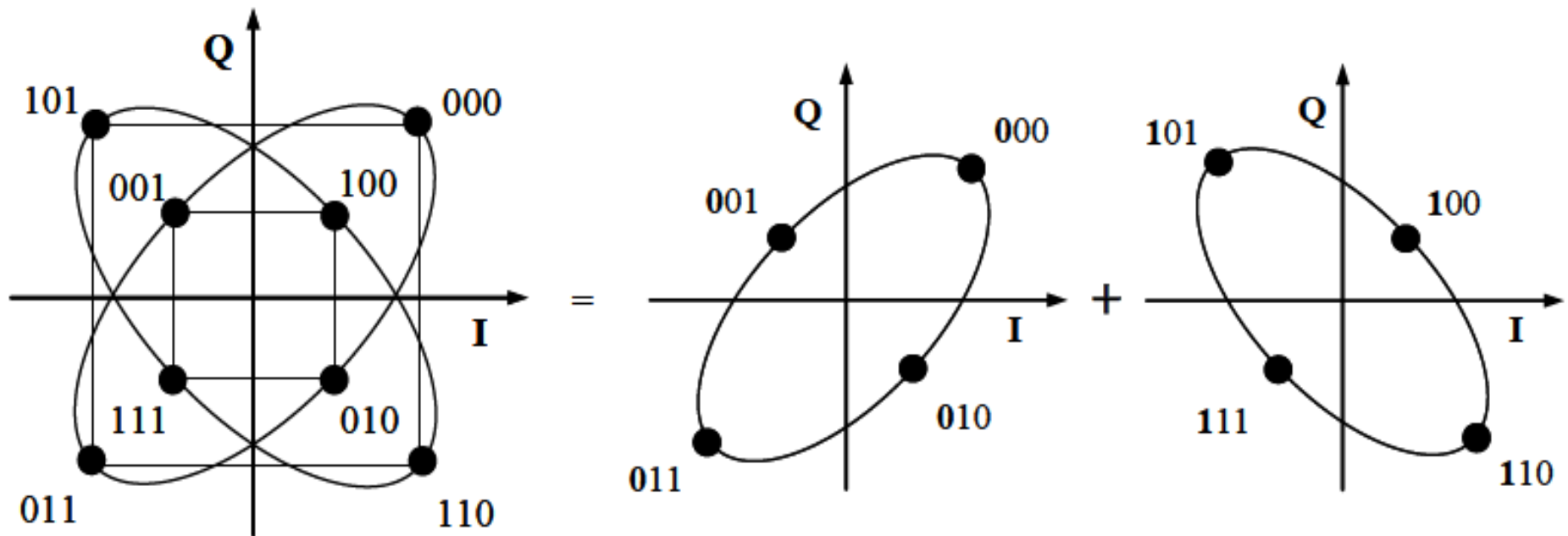
Constellation of 8-EPSK signals
